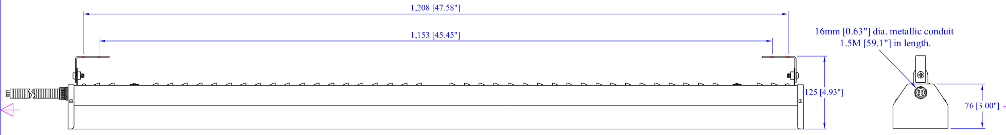
SIDE VIEW WITH MOUNTING BRACKETS ASSEMBLED
