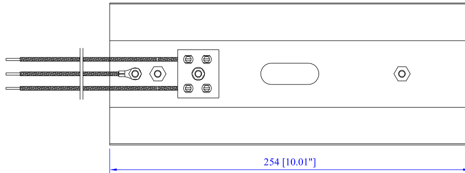
REAR VIEW
