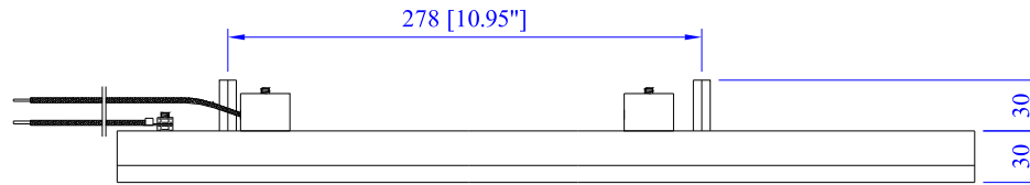
SIDE VIEW
