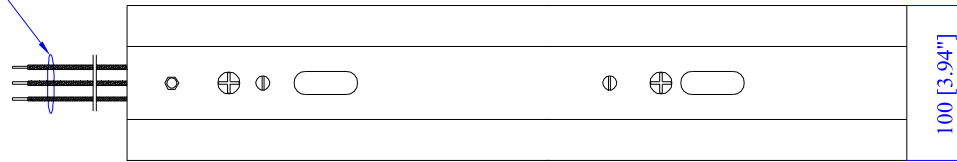
FRONT VIEW
