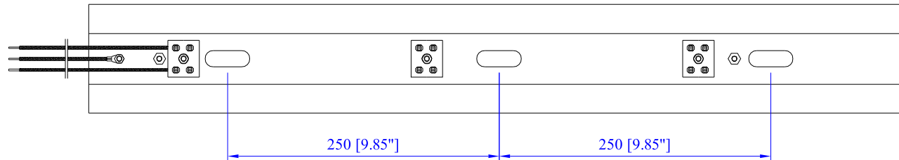
TOP VIEW
