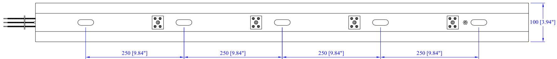
TOP VIEW
